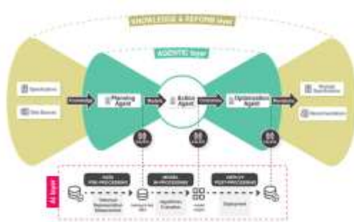
Fig 4: Agentic AI fairness framework
